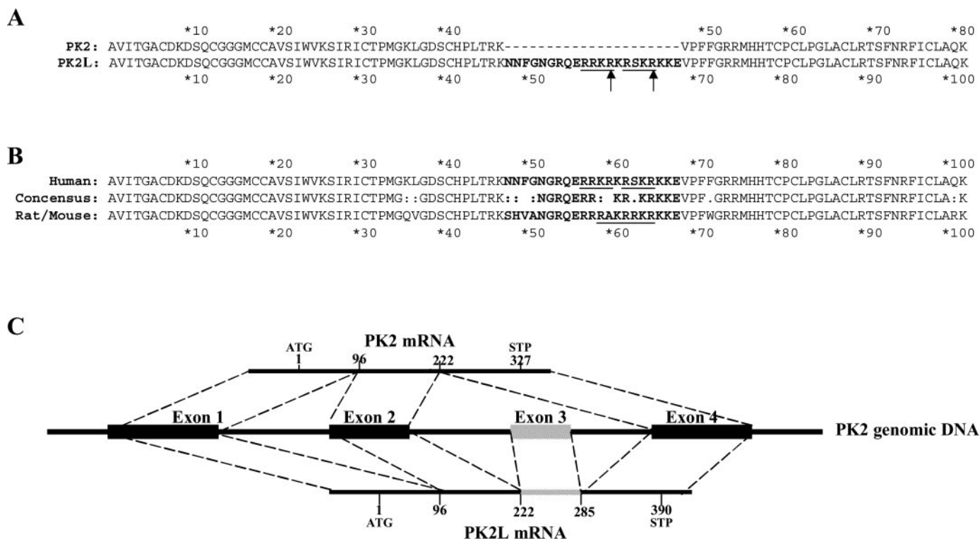
Fig. 1. A, amino acid sequence comparison between human PK2 and PK2L (without signal peptide). The 21 additional amino acids in PK2L are highlighted in bold letters. The furin recognition sequences are underlined. The potential furin cutting sites are indicated by arrows. B, amino acid sequence comparison between human and rat/mouse PK2L. Rat and mouse PK2L are identical. The putative furin recognition sequences are underlined. C, gene structure of PK2 and the differential exon use by PK2 and PK2L mRNA. The numbers indicate the nucleotide positions in PK2 and PK2L coding regions, respectively. ATG and STP represent the translation start and stop codons, respectively.
