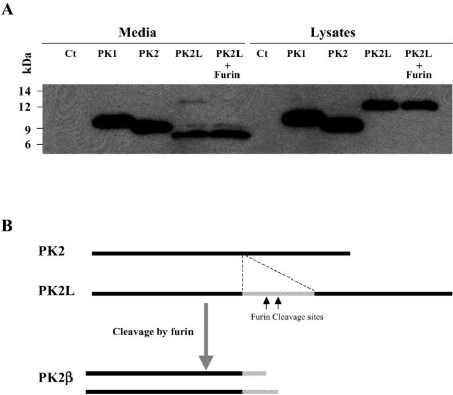
Fig. 3. A, Western blot analysis of recombinant PKs expressed in COS-7 cells. N-terminal FLAG-tagged PK1, PK2, and PK2L either from cell-conditioned media or from cell lysates were analyzed by Western blot using anti-FLAG M2 antibody. B, schematic for PK2, PK2L, and PK2β. The 21-amino acid insertion in PK2L is shown in hatched box. The putative furin cleavage sites are indicated with arrows.
